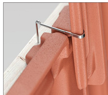
All clay and concrete roof tiles should be mechanically fixed.
