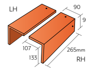
Cloaked verge tiles
