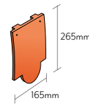
Club feature tile
